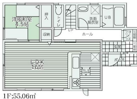
1F:55.06㎡
